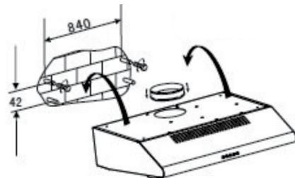
90cm hood
