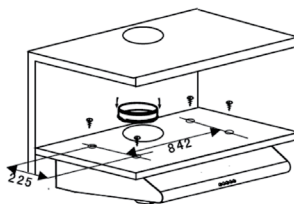
90cm hood
